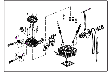
CYLINDER HEAD ASSEMBLY Fig. No. 04, Page No. 24
