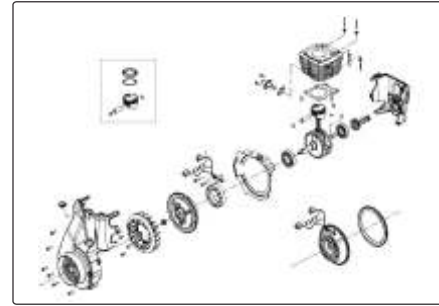
CYLINDER BLOCK & PISTON ASSEMBLY Fig. No. 03, Page No. 22
