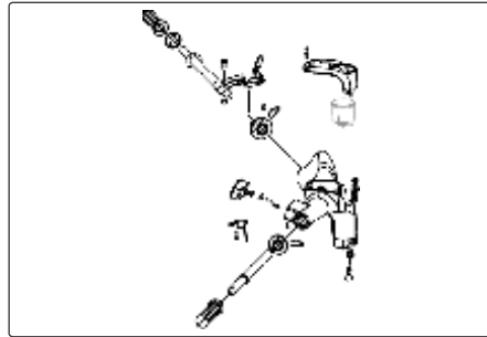
HANDLE BAR ASSEMBLY Fig. No. 14, Page No. 50
