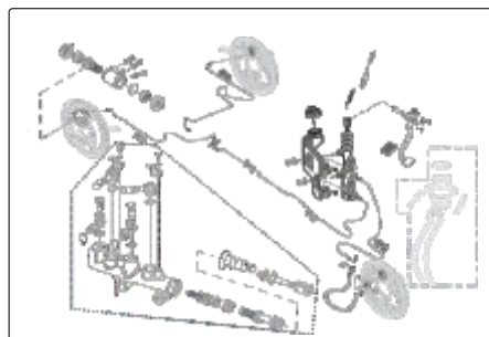
HYDRAULIC BRAKE SYSTEM Fig. No. 21, Page No. 68
