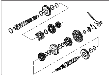
GEAR BOX ASSEMBLY Fig. No. 05, Page No. 28
