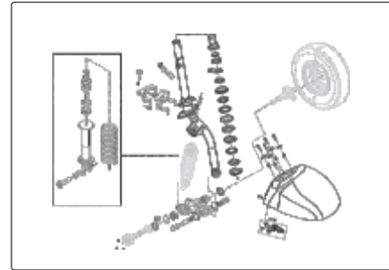
FRONT FORK ASSEMBLY Fig. No. 15, Page No. 52
