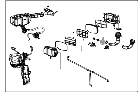
INDUCTION SYSTEM Fig. No. 08, Page No. 34
