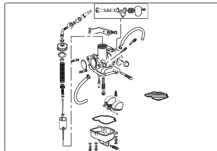
CARBURETOR ASSEMBLY Fig. No. 10, Page No. 40
