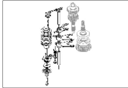
GEAR SHIFTER MECHANISM Fig. No. 06, Page No. 30
