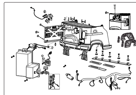
PASSENGER BODY & ELECTRICALS Fig. No. 23, Page No. 72
