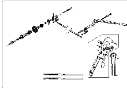
HAND STARTER & PARKING BRAKE MECHANISM Fig. No. 17, Page No. 58
