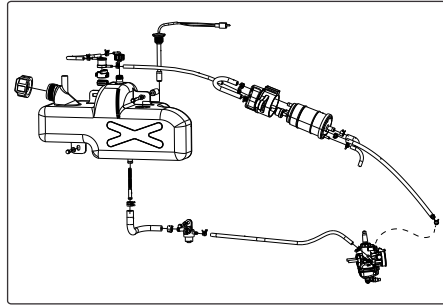
FUEL TANK & CANISTER SYSTEM - BSIV Fig. No. 13, Page No. 48
