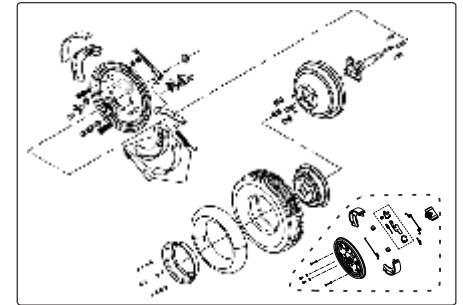
REAR WHEEL ASSEMBLY Fig. No. 20, Page No. 66
