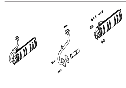
MUFFLER ASSEMBLY Fig. No. 11, Page No. 44
