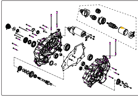
CRANK CASE ASSEMBLY Fig. No. 01, Page No. 14
