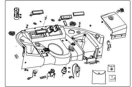
DASH BOARD ASSEMBLY Fig. No. 16, Page No. 56
